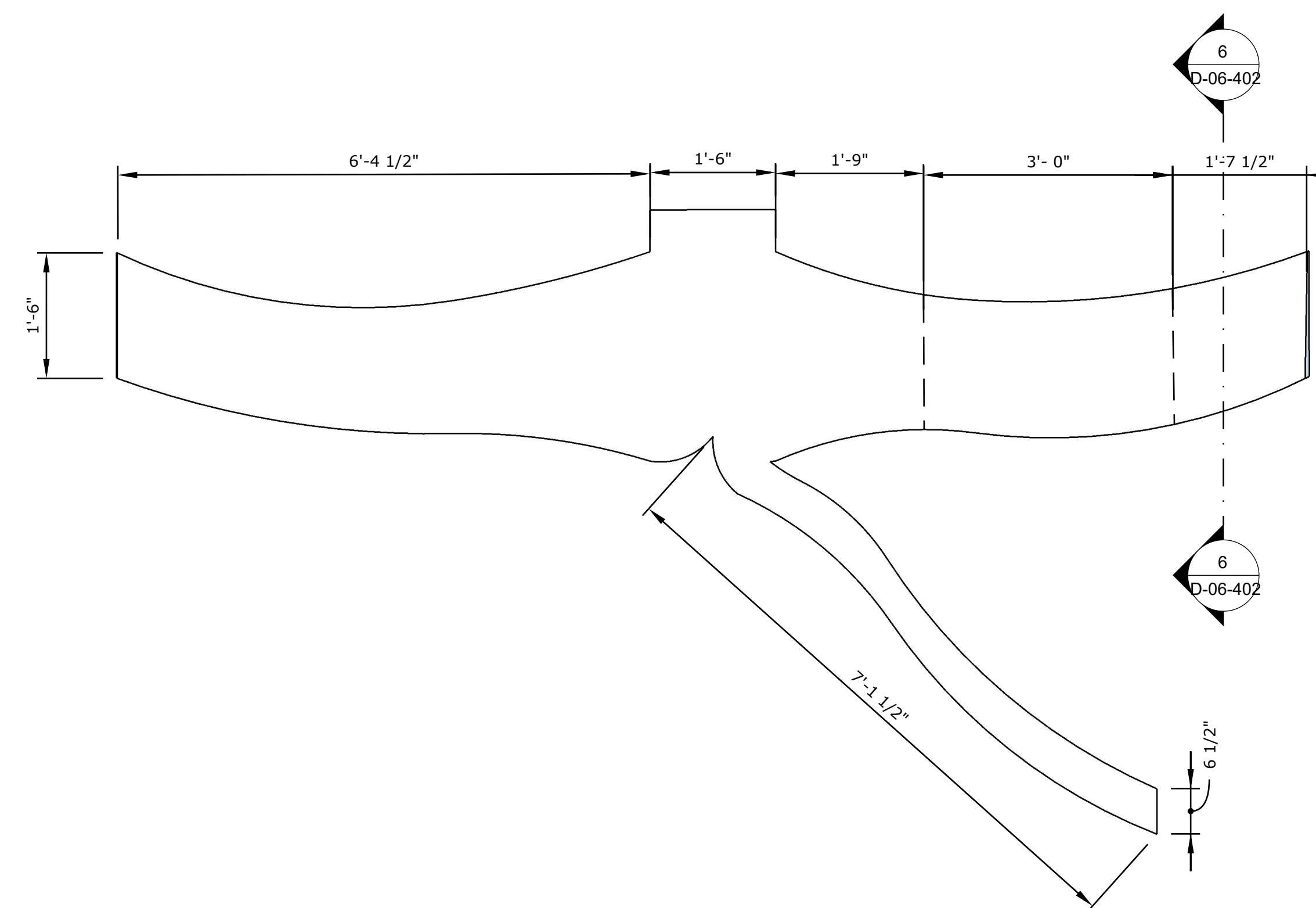
ANIMATRONIC BOOK - TOP VIEW
