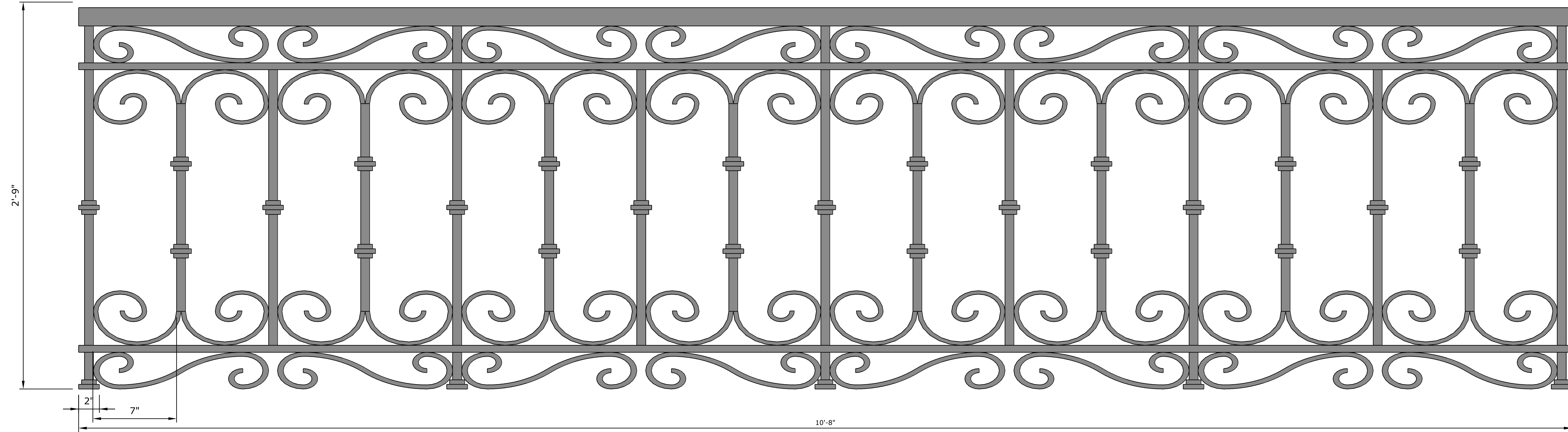
1 FRONT VIEW: VICTORIAN RAILING D-01-501 SCALE: 3" = 1'-0"
