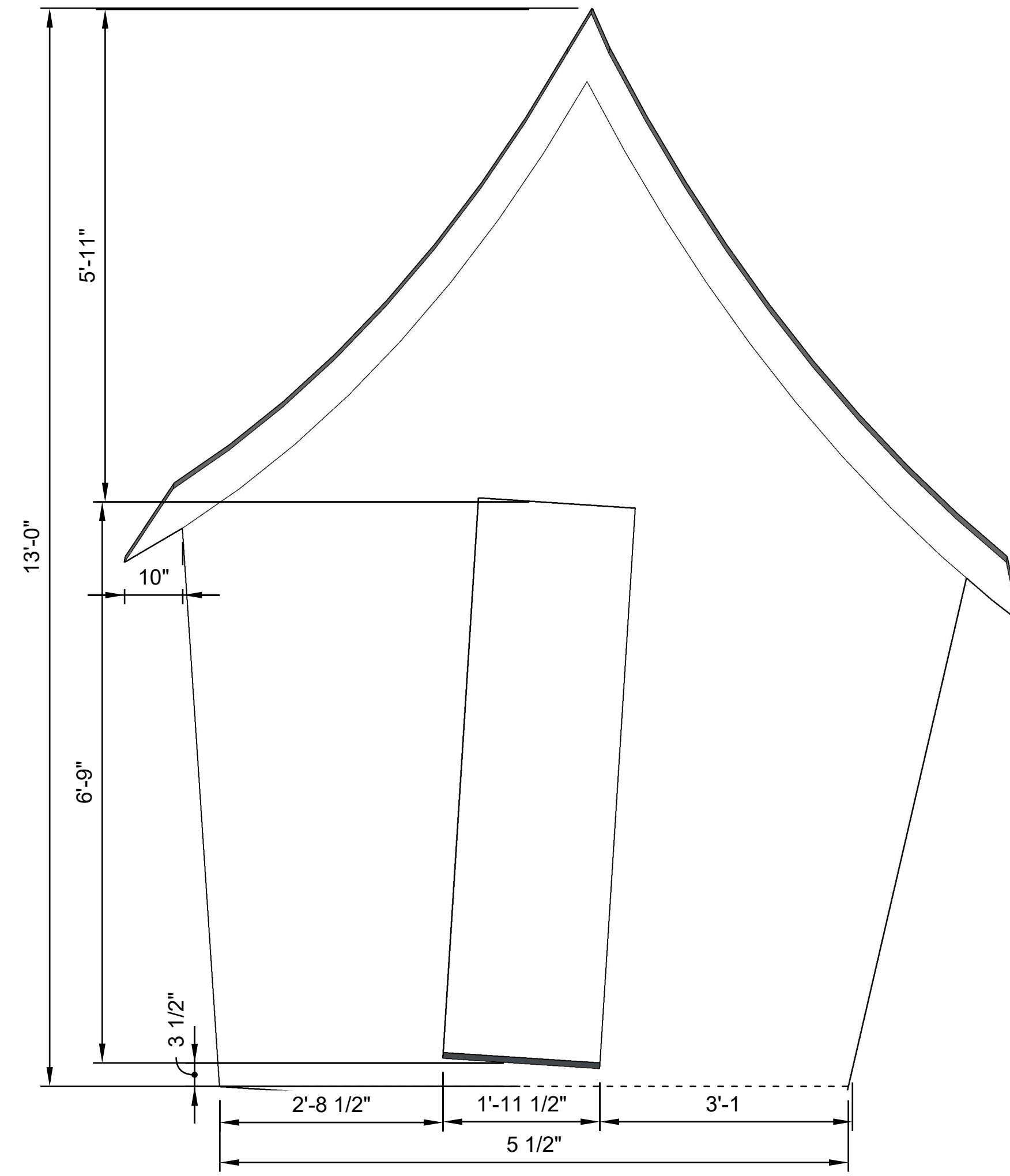
ANNE'S SHED - ELEVATION
