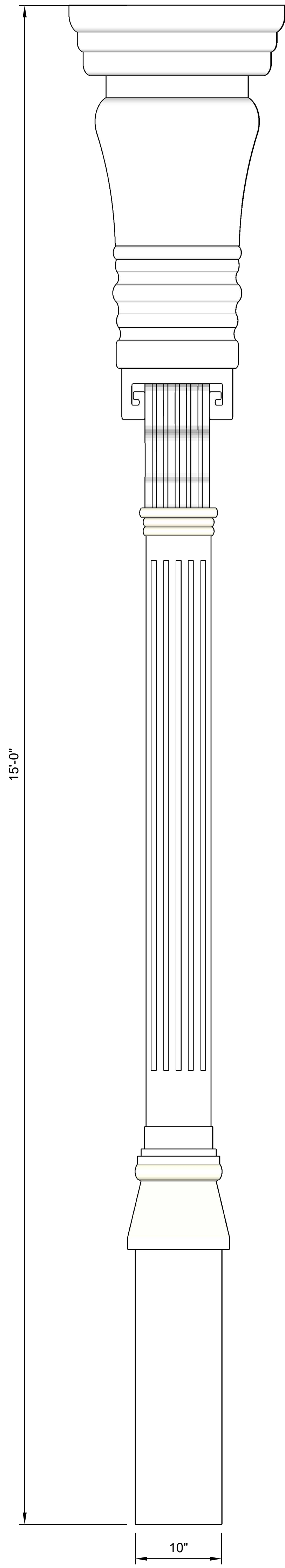
1 FRONT VIEW: VICTORIAN COLUMN D-01-502 SCALE: 1 1/2" = 1'-0"
